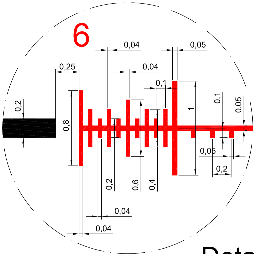
Detail A
