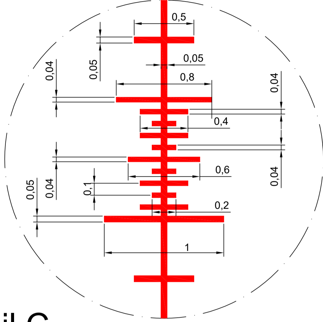
Detail B
